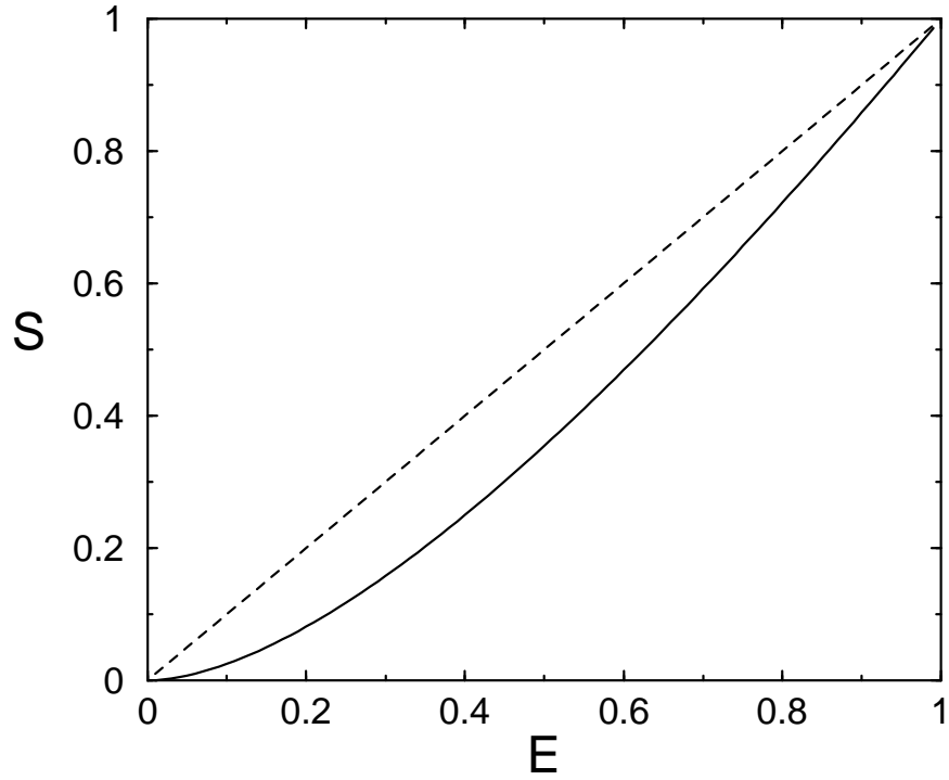
FIG. 2. The entropy of entanglement S (solid line) in terms of the measure of entanglement E for a pure spin-1/2 entangled state. The dashed line is an eye-guidance for a linear curve. The entropy of entanglement S is a monotonously increasing function of the measure of entanglement E for a pure state because the first derivative of S is positive everywhere from 0 to 1 of E .
