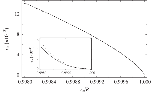
FIG. 3. Dependence of the energy \epsilon_n (main plot) and width \gamma_n (inset) of the n = 6 resonance on r_s for the Florides interior metric. Solid circles show the numerical values and solid lines show the results obtained from Eqs. (17) and (18) using B(\xi) from Eq. (28).
