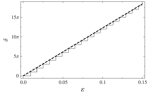
FIG. 4. Short-range phase \delta obtained for the Soffel interior metric for r_s/R = 0.955 (solid line), and the interior phase \Phi = \epsilon r_s B(\xi) (dashed line), with B(\xi) given by Eq. (30).
